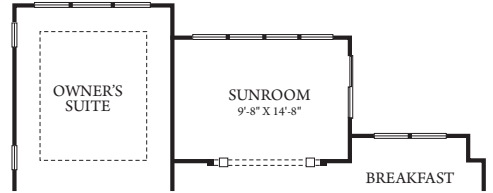
OPT. SUNROOM
